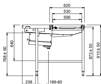
Factory mounted waste rack
